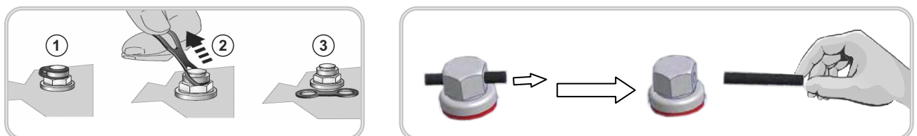
Figure 3: Activation of Vent Plug
