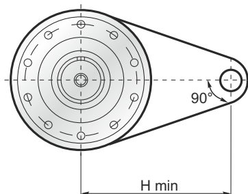
Figure 13: Torque Arm
