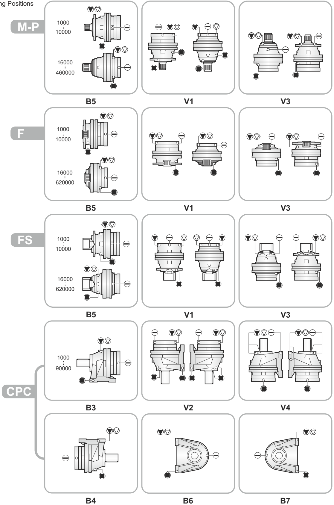
Figure 10: Mounting Positions
